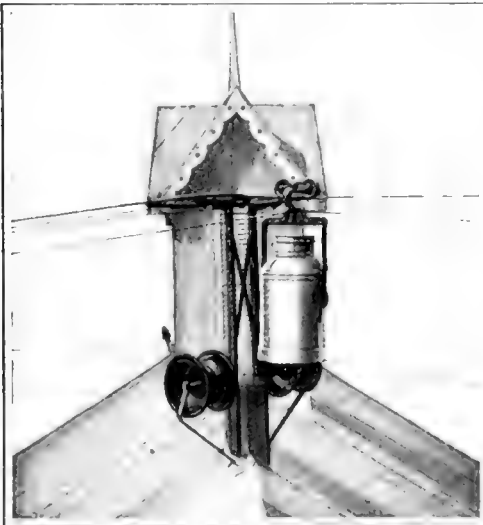
The apparatus in position, showing the carrying and traction cables. Two cans are always in transit
